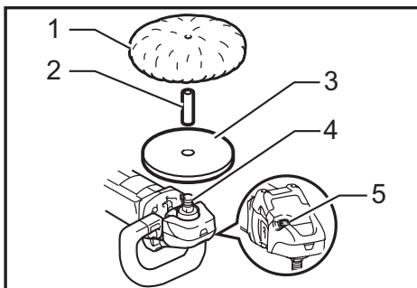
► 1. Wool pad 2. Sleeve 18 3. Backing pad 4. Spindle 5. Shaft lock
