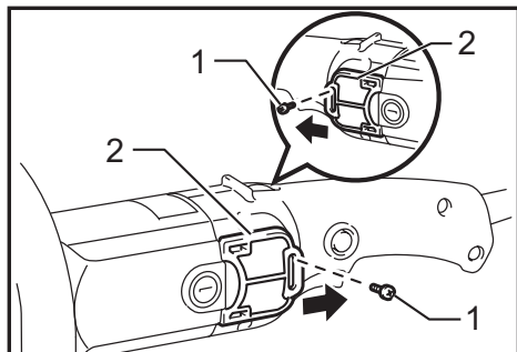
► 1. Screw 2. Dust cover
